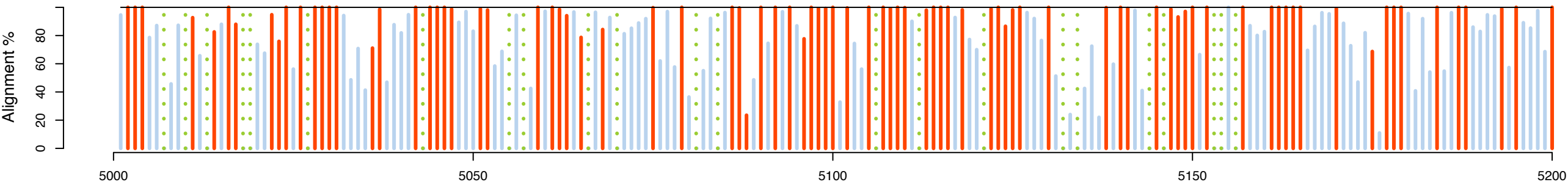
Gene set: tribcas4a (75% ref align, 43% best)
