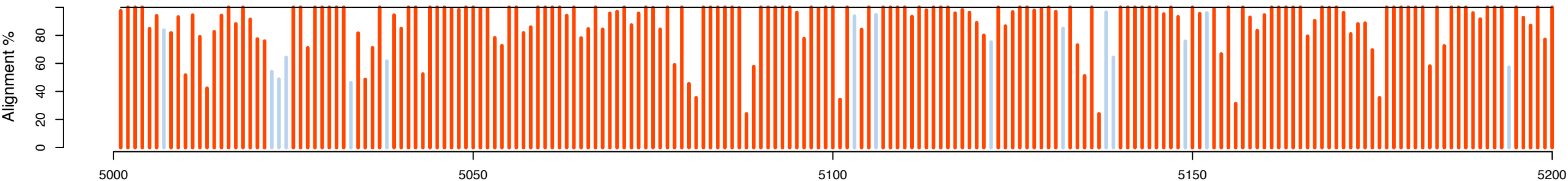
Gene set: tribcas4evg2 (89% ref align, 92% best)
