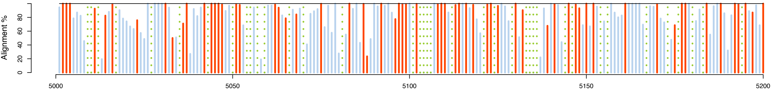
Gene set: tribcas1 (69% ref align, 32% best)
