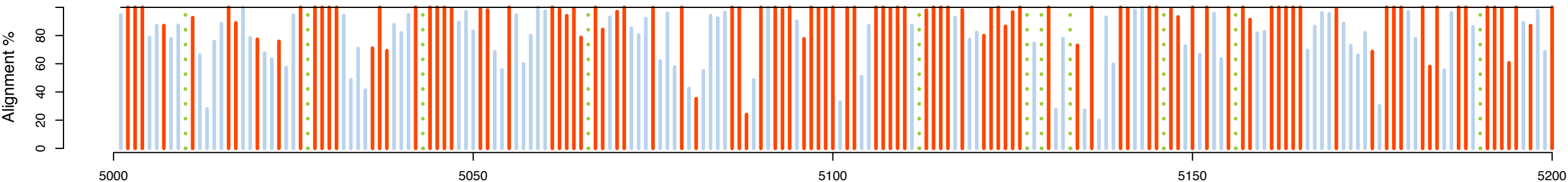
Gene set: tribcas14nc (82% ref align, 52% best)
